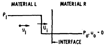
(a) PRESSURE-DISTANCE PROFILE BEFORE INTERACTION
